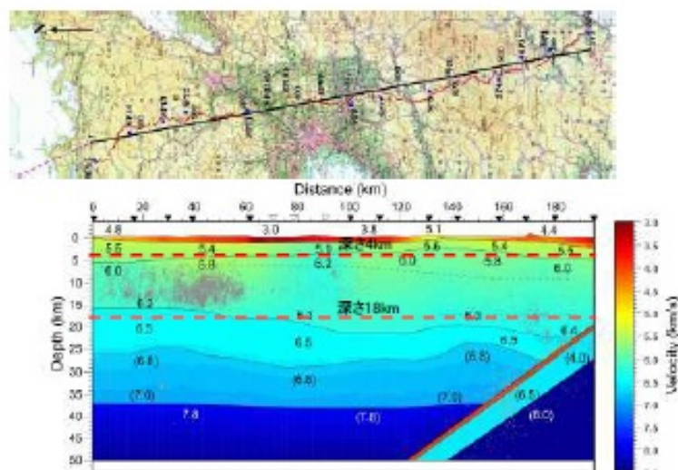
Fig. 9 P-wave velocity structure for the. Numerals show P-wave velocities in km/s. Parentheses show assumed velocity values. Small black and red dots (about 35-40km deep) show earthquakes and low-frequency earthquakes, respectively after Hase and Ito (2007).
